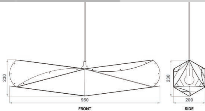
Stainless Steel
